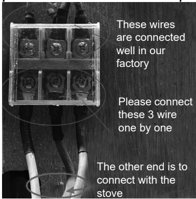
3-wires cable
