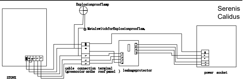
380v wiring diagram LM-T03B LM-T03A
